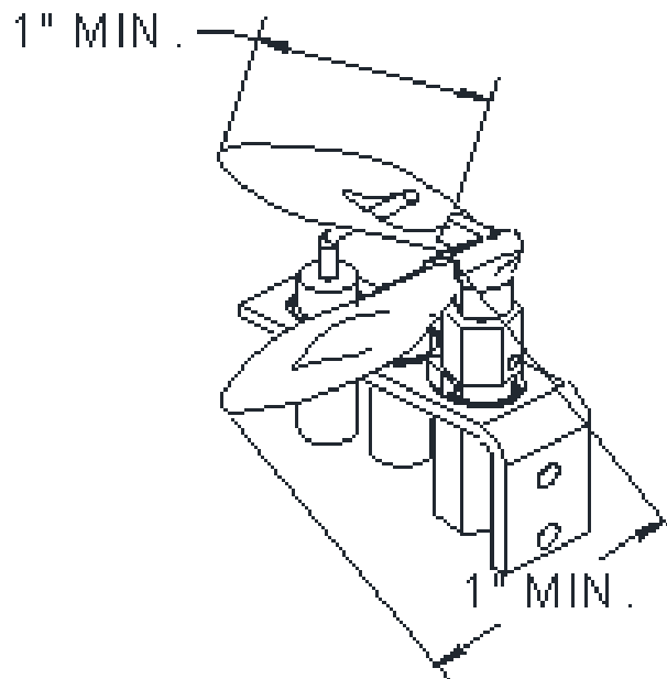
Pilot Flames
